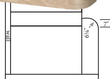
8040 Single End Quarter Circle Starting Step 11¼" x (varies)*
